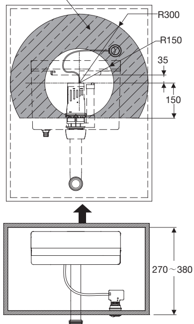
Push Button Installation Area
