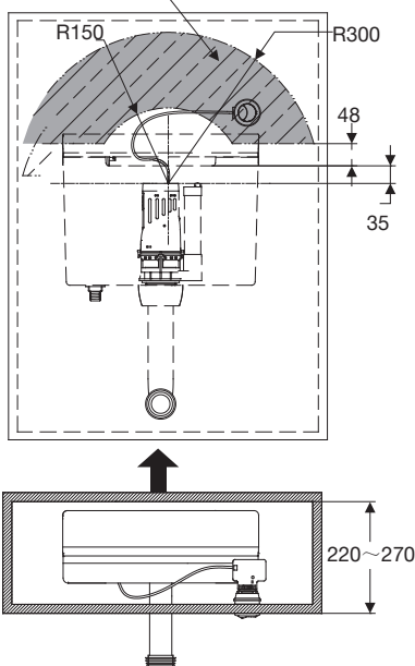
Push Button Installation Area
