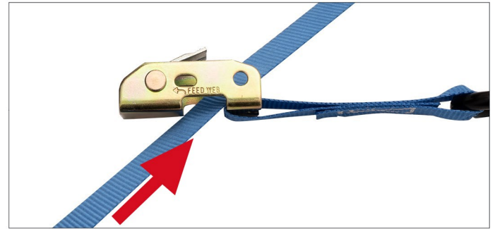
1 Feed approximately 20cm of the long webbing strap up and through the cam buckle in the direction of the arrow shown above.
