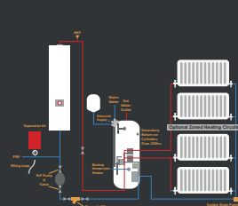
Heating and Hot Water Design with Pre-Plumbed Indirect Cylinder
