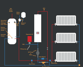
Heating and Hot Water Design with Indirect Cylinder
