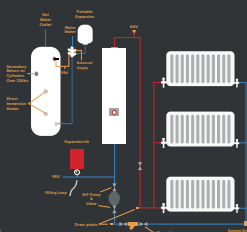
Heating Only with Direct Cylinder Hot Water Design
