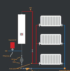
Heating Only Design
